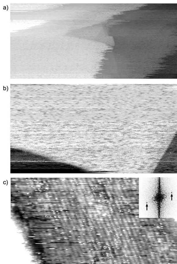
Figure 3. STM of the Ag(111) surface under reaction conditions. The reaction gas mixture was 0.5 mbar of ethylene and 0.5 mbar of \text{O}_2 , T = 470 \text{ K} . a) 1000 \text{ Å} \times 450 \text{ Å} , +1.0 \text{ V} , 0.3 \text{ nA} ; b) 490 \text{ Å} \times 260 \text{ Å} , +1.0 \text{ V} , 3.0 \text{ nA} ; c) 250 \text{ Å} \times 130 \text{ Å} , +1.0 \text{ V} , 1.0 \text{ nA} . Inset: Fourier transform of the image.
